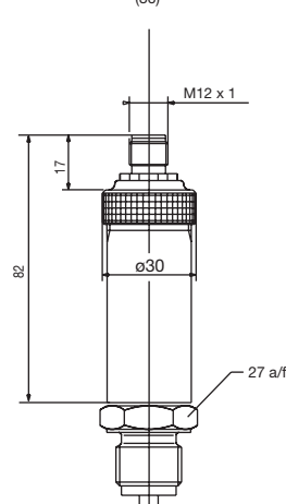
Electrical connection with circular connector M12 x 1 (36)
