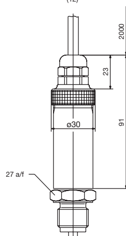
Electrical connection with attached cable (12)
